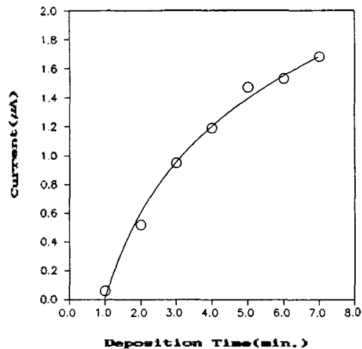
Fig. 5. Dependence of the SWASV peak current on the deposition time for 10 ppb mercury solution.
