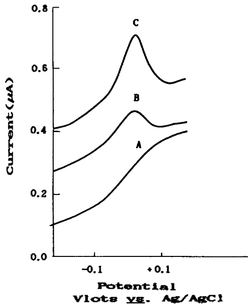
Fig. 1. Dependence of the SWASV peak current on the stirring rate for 1 ppb mercury solution. A; non-stirring, 1 ppb. B; Stirring at 400 rpm, 1 ppb(210 nA). C; Stirring at 700 rpm, 1 ppb (433 nA).
