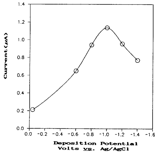
Fig. 2. Effect of deposition potential on the SWASV peak current for 10 ppb mercury solution.
