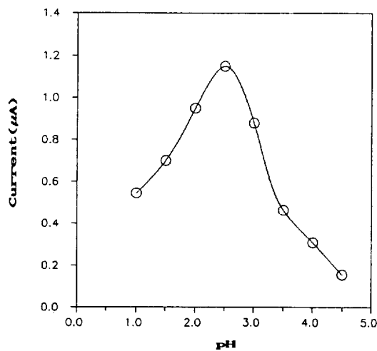
Fig. 3. Effect of pH on the SWASV peak current for 10 ppb mercury solution at the deposition time 240 sec.
