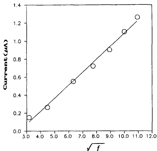
Fig. 4. Effect of frequency (Hz) on the SWASV peak current for 10 ppb mercury solution.
