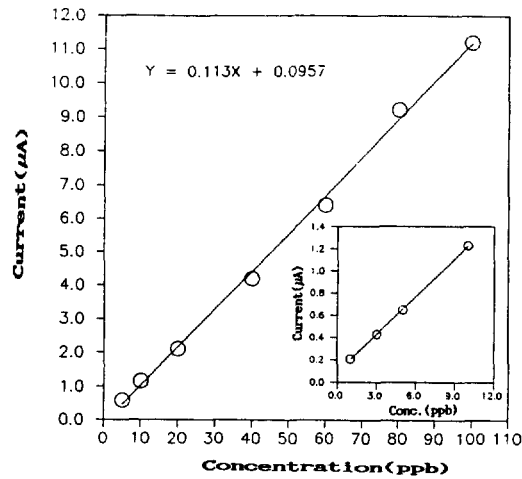
Fig. 7. Calibration curve for the square wave anodic stripping voltammetric determination of mercury in 0.1M KSCN solution. pH, 2.5; Deposition time, 240 sec; Deposition potential, -1.0 V; Frequency, 100 Hz; Stirring rate, 400 rpm.
