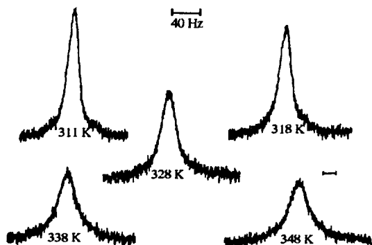
Fig. 2. ^1\text{H} -NMR spectra of 0.5 m NEAA amide proton in n -pentanol solvent at various temperature.
