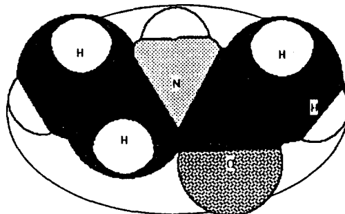
Fig. 4. Molecular structure of N-ethylacetamide. The solid ellipse represents outlines of the prolate ellipsoid used to model the solute shape.
