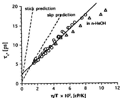
Fig. 3. Dependence of the reorientational correlation time \tau_c of NEAA on viscosity \eta (cP) divided by absolute temperature T (K) in n -alcohol solvents. The solid line represents the linear best fit up to the n -PeOH data. The stick and slip predictions are shown by dashed lines.
