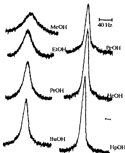
Fig. 1. 1 H-NMR spectra of 0.5 m NEAA amide proton in n -alcohol solvents at 313 K.
