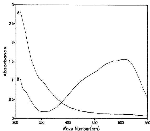
Figure 1. UV-VIS spectrum of iron-phenanthroline complex from A; Crude 2-HEMA products from FeCl 3 ·6H 2 O+NaNO 3 system, B; Crude 2-HEMA products from FeCl 3 ·6H 2 O+PMP system. Condition; 1% (v/v) of crude 2-HEMA in potassium acetate-acetic acid buffer (1×10 -2 M, pH 4), [Phenanthroline]=2×10 -4 M.
