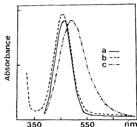
Figure 1. Visible absorption spectra of (a) [NiL 2 ] 2+ in CH 3 NO 2 , (b) [NiL 3 ] 2+ in CH 3 CN, and (c) [CuL 3 ] 2+ in CH 3 NO 2 at 25°C. [Notice the absence of the characteristic octahedral Ni(II) band of around 350 nm in CH 3 CN solution.]
