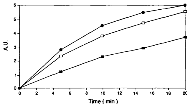
Figure 6. Effect of enzyme concentration with different reaction on the formation of product. The reaction mixture was 1% soluble starch in 0.1 M Tris-HCl (pH 8.0) 50 ml and (■) 1 unit/ml enzyme, (□) 2 units/ml enzyme solution 100 \mu l, (○) 3 units/ml of enzyme were incubated at 37°C for 5 min, 10 min, 15 min, 20 min. Liberated maltoheptaose was measured by DNS assay method.
