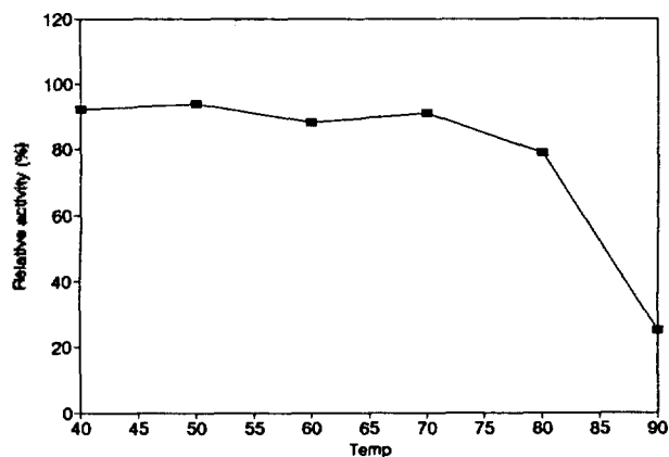
Figure 11. Thermostability test of \alpha -amylase with 1 mM CaCl_2 at pH 8.0.
