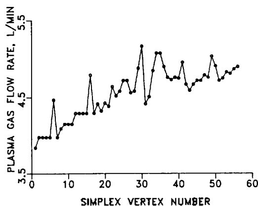
Figure 12. Movement of the plasma gas flow rate as a function of the simplex vertex number.
