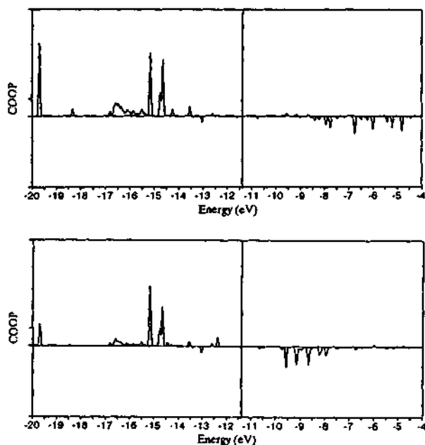
Figure 5. (a) COOP curve of C-S bond when the 1,3,5-trithian is adsorbed on on-top site. (b) Contribution S 3p x to this C-S bond. The vertical line around -11.5 eV represents the Fermi energy.
