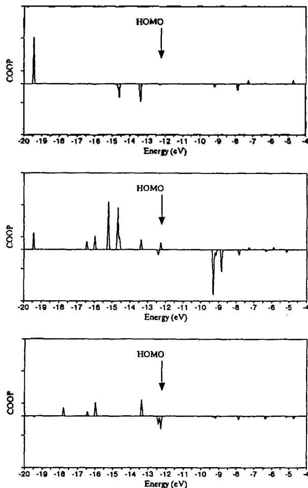
Figure 3. Resolved COOP curve of C-S bond of free 1,3,5-trithian molecule. (a) Contribution of S 3s atomic orbital. (b) Contribution of S 3p x (S 3p x +S 3p y ) atomic orbital. (c) Contribution of S 3p z (S 3p z ) atomic orbital.
