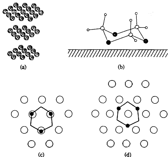
Figure 1. (a) The geometry of the \text{Ag}_{43} (19, 12, 12) cluster used in this study. (b) The adsorption geometry of 1,3,5-trithian molecule on Ag surface. (c) On-top site adsorption. Large white circles denote 1st layer Ag atoms and small black circles Sulfur atoms. (d) 3-fold site adsorption.
