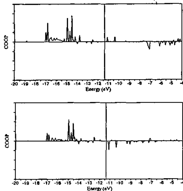
Figure 6. (a) COOP curve of C-S bond when the 1,3,5-trithian is adsorbed on 3-fold site. (b) Contribution S 3p_x to this C-S bond. The vertical line around -11.5 eV represents the Fermi energy.
