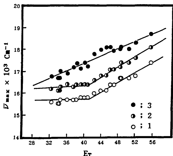
Figure 1. Plots of frequency \nu_{\max} \times 10^3 vs. E_T for the open-chain merocyanine form of 5-chlorinated 1,3,3-trimethylindolinobenzospiropyrans; 1 (○); 2 (◐); 3 (●), in various solvents.
