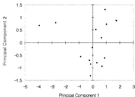
Fig. 2. Principal component score plot of exchangeable fraction in the surface sediments of Ulsan Bay.
