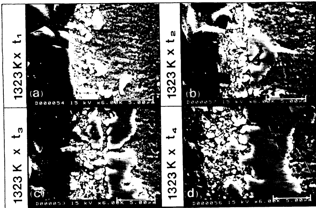
Photo. 8 SEM micrographs for the illustration of the Sequence of Reactions to form layer I and II in a \text{Al}_2\text{O}_3/\text{Cu-7.5wt\% Zr/STS304} System ( t = \text{Bonding time} , t_1 < t_2 < t_3 < t_4 )
