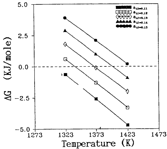
Fig. 4 Free Energy change of Interfacial Reaction in the \text{Al}_2\text{O}_3/\text{Cu-7.5wt\% Zr/STS304} System as a Function of Activities of Aluminum
