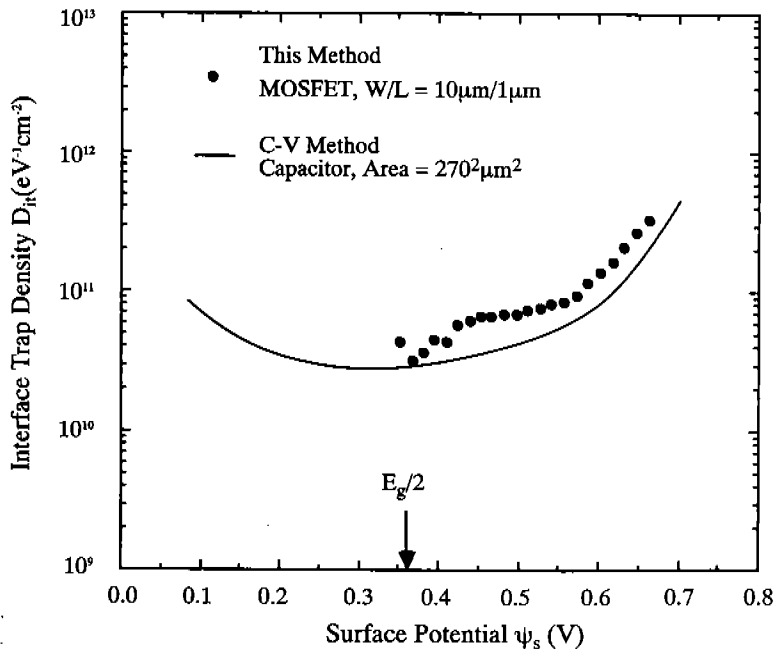
Fig. 8. The energy distribution of interface traps in the band gap for the n-MOSFET through the subthreshold slope measurement (•) and that for a capacitor through the C-V method (—).
