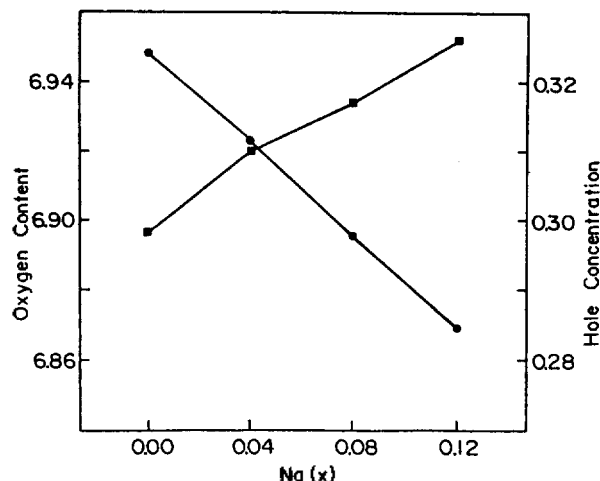
Figure 5. Oxygen content (●) and hole concentration (■) vs. Na content for Y_{1-x}Na_xBa_2Cu_3O_{7-x} compounds. Errors associated with measured oxygen contents are estimated to be \pm 0.01 .
