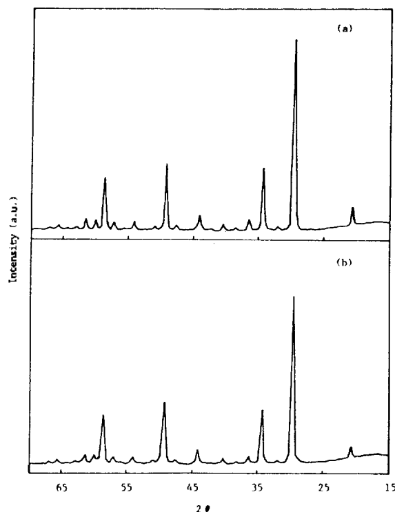
Figure 1. X-ray diffraction patterns of 1(a) and 9 mol% (b) \text{ZrO}_2 -doped \text{Yb}_2\text{O}_3 system.
