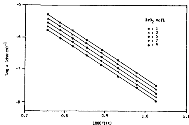
Figure 6. Temperature dependence of electrical conductivity of various ZrO 2 -doped Yb 2 O 3 samples under 2 \times 10^{-1} atm oxygen partial pressure.
