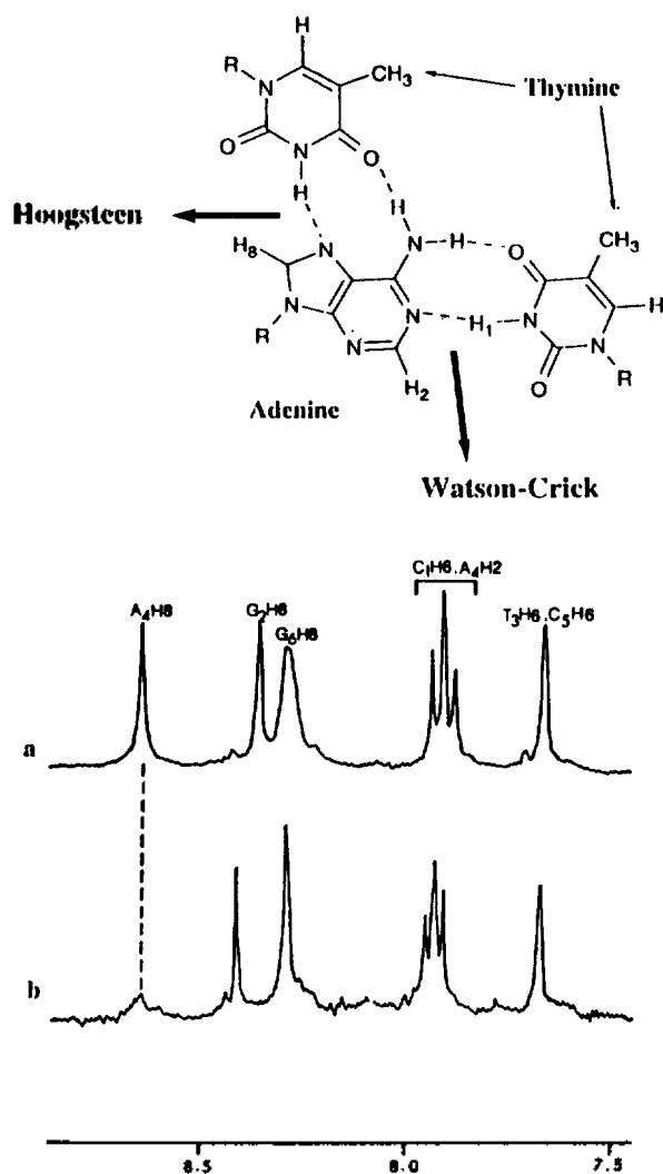
Figure 1. (a) 500 MHz ^1\text{H-NMR} spectrum of the aromatic proton resonances of the d(\text{CGTACG}) duplex obtained in \text{D}_2\text{O} buffer, pH 7.0, 25^\circ\text{C} . Assignments of some of the DNA resonances are indicated on the figure. (b) Spectrum of DNA hexamer deuterated at the adenine H-8 position; otherwise similar to (a) Dotted line connect resonance position of the adenine H-8 proton. (Inset) Standard A. T and Hoogsteen A. T base pairs. The imino, H-2, and H-8 protons are designated \text{H}_1 , \text{H}_2 , and \text{H}_8 , respectively.
