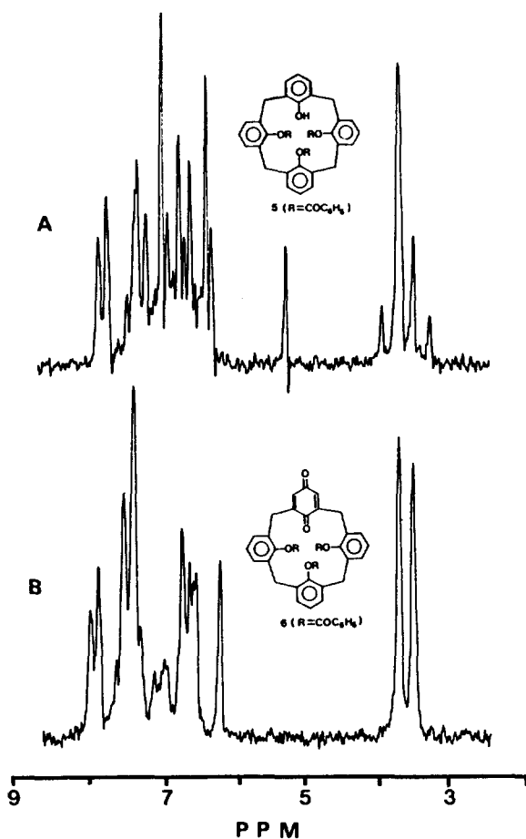
Figure 2. Proton NMR spectra of 5 and 6.
