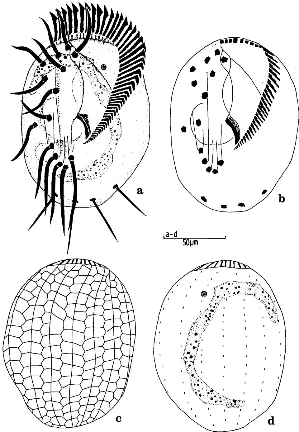
Fig. 2. Euplotes aediculatus Pierson : a, entire ventral view of living specimen; b, infraflagellate in ventral view after protargol impregnation; c, dorsal silver line after wet silver impregnation; d, dorsal kineties and nuclear arrangement after protargol and wet silver impregnation.
