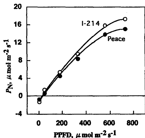
Fig. 1. Photosynthetic response to irradiance of two poplar clones grown under 350 \mu\text{L L}^{-1} \text{CO}_2 . Measurements were made at 350 \mu\text{L L}^{-1} \text{CO}_2 .
