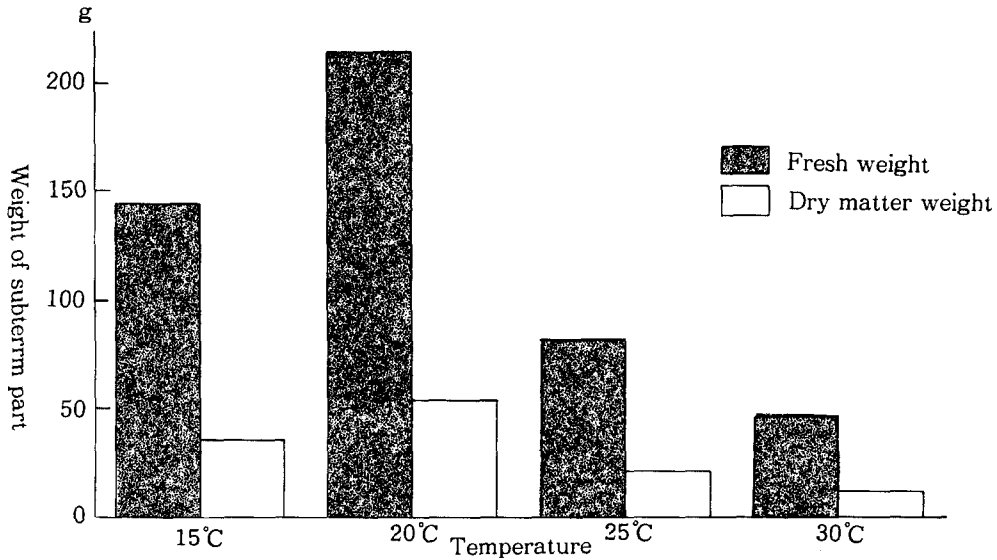
Fig. 3. The effect of subterranean part weight with different temperature in C. lanceolata
