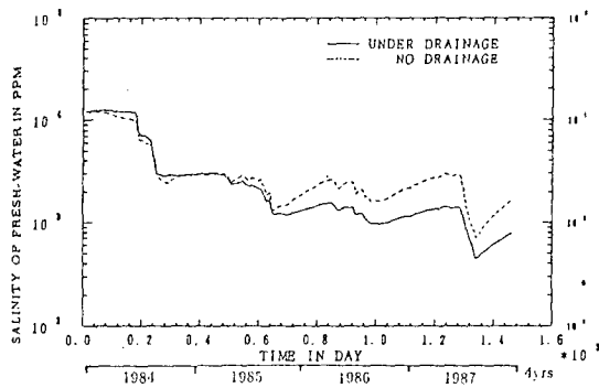
Fig. 10 Salinity of freshwater layer in the Dai-ho reservoir
