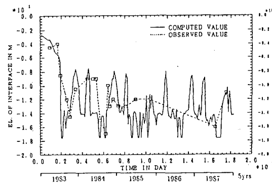
Fig. 17 Interface variation for the Nam-yang reservoir
