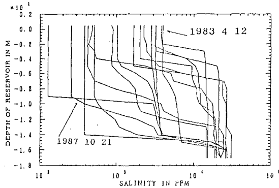
Fig. 4 Observed salinity distribution at the Nam-yang reservoir.
