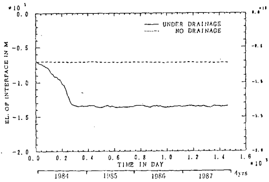
Fig. 11 Interface water level in the Dai-ho reservoir
