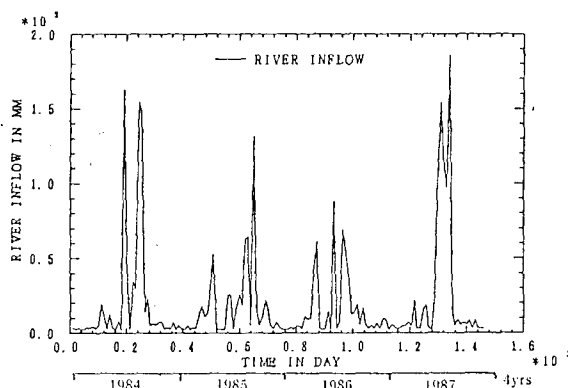
Fig. 9 Inflow for the Dai-ho reservoir.
