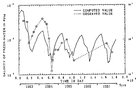
Fig. 16 Salinity variation for the Nam-yang reservoir
