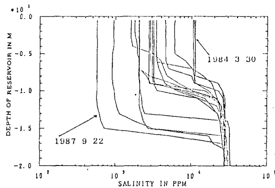
Fig. 5 Observed salinity distribution at the Dai-ho reservoir.
