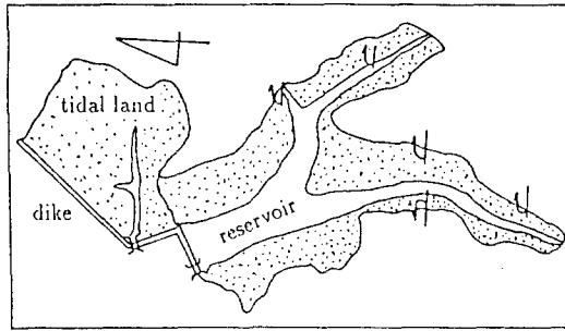
Fig. 3 Map showing of the Dai-ho project
