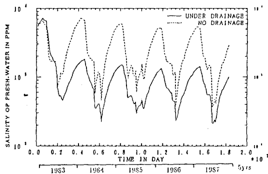
Fig. 12 Salinity of freshwater layer in the Nam-yang reservoir
