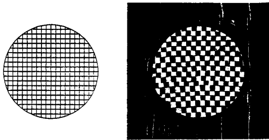
(a) Before deformation.
