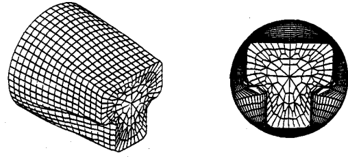
(b) Reduction of area:50%
