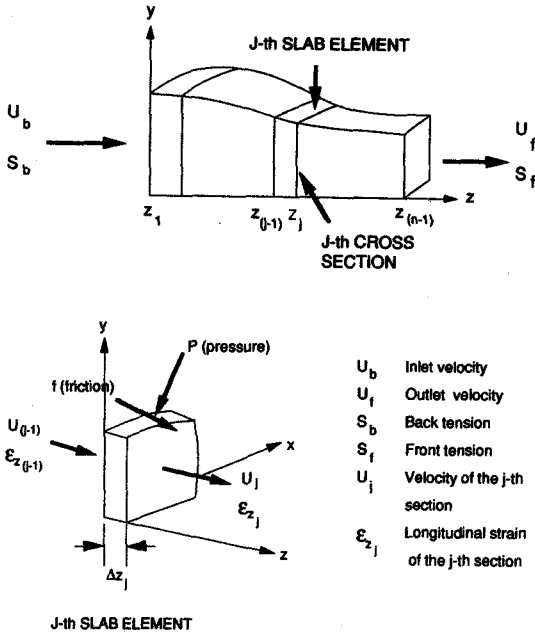
Fig. 1. Application of finite and slab element method to extrusion processes.
