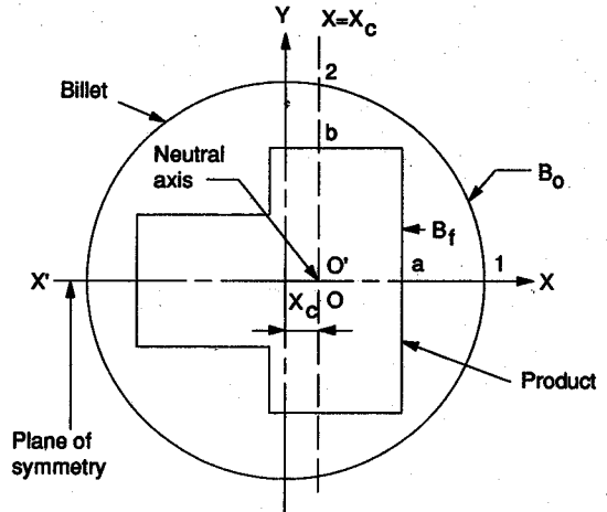
(a) Determination of the neutral axis.
