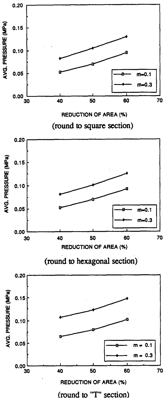
Fig. 13. Influence of reduction of area and friction factor on the extrusion pressure.
