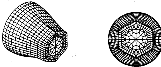
(c) Reduction of area:60%
