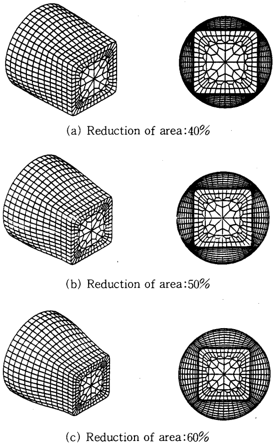
Fig. 6. Grid distortions to the various reduction of area(round to square section).
