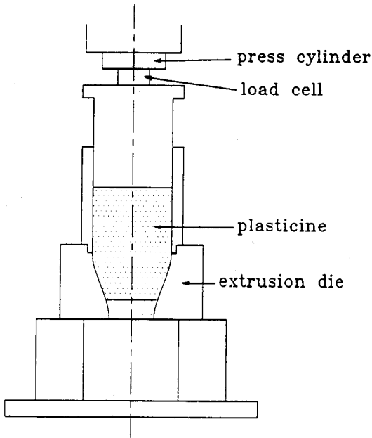
Fig. 5. Schematic diagram of experimental equipment.
