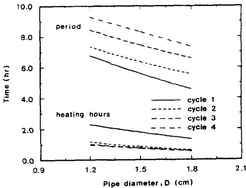
Fig.11 Period and heating hours per cycle with various pipe diameters
