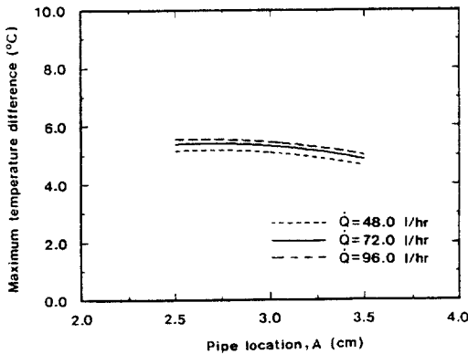
Fig. 10 Maximum temperature differences at panel surface for various pipe locations and flow rates
