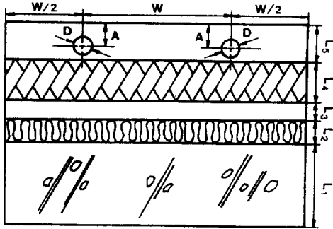
Fig.1 Model of radiant heating panel for the typical level
