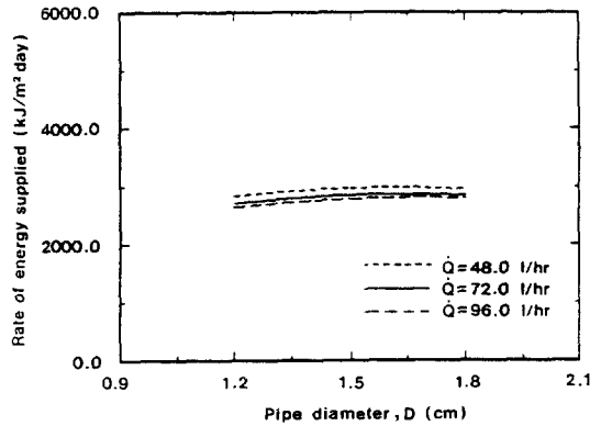
Fig.13 Rates of energy supplied per day per unit panel surface area for various pipe diameters and flow rates
