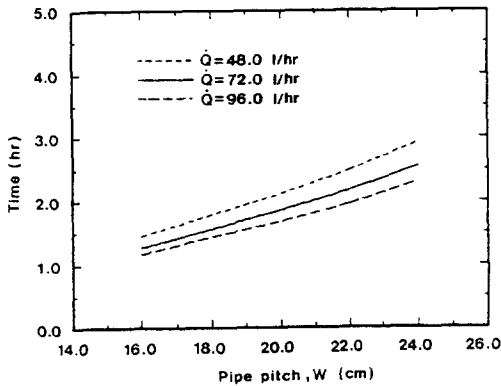
Fig. 4 Total heating hours per day for various pipe pitches and flow rates
