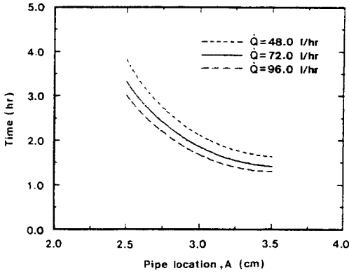
Fig. 8 Total heating hours per day for various pipe locations and flow rates
