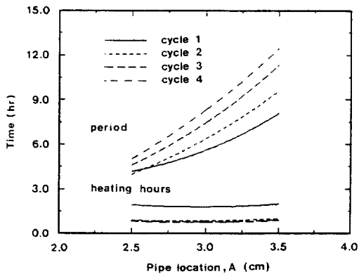
Fig. 7 Period and heating hours per cycle with various pipe locations
