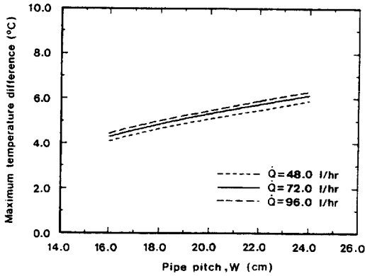
Fig. 6 Maximum temperature differences at panel surface for various pipe pitches and flow rates
