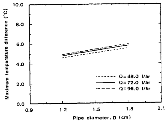
Fig.14 Maximum temperature differences at panel surface for various pipe diameters and flow rates
