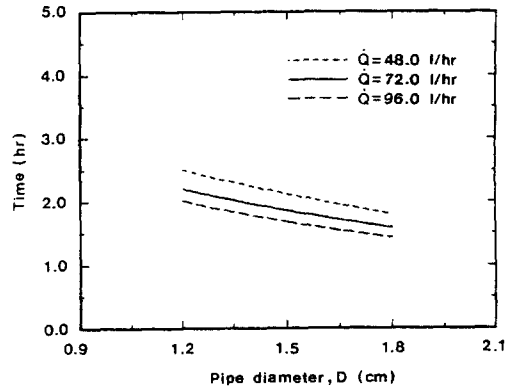
Fig.12 Total heating hours per day for various pipe diameters and flow rates
