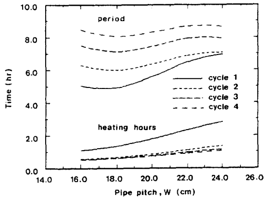
Fig. 3 Period and heating hours per cycle with various pipe pitches
