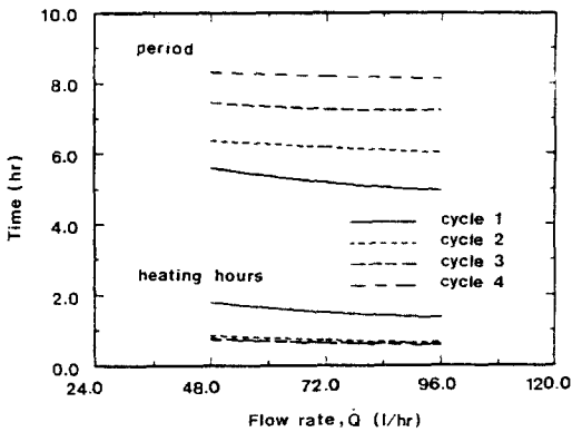
Fig. 2 Period and heating hours per cycle with various flow rates
