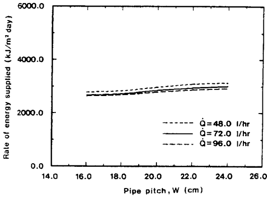
Fig. 5 Rates of energy supplied per day per unit panel surface area for various pipe pitches and flow rates
