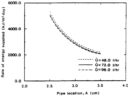
Fig. 9 Rates of energy supplied per day per unit panel surface area for various pipe locations and flow rates
