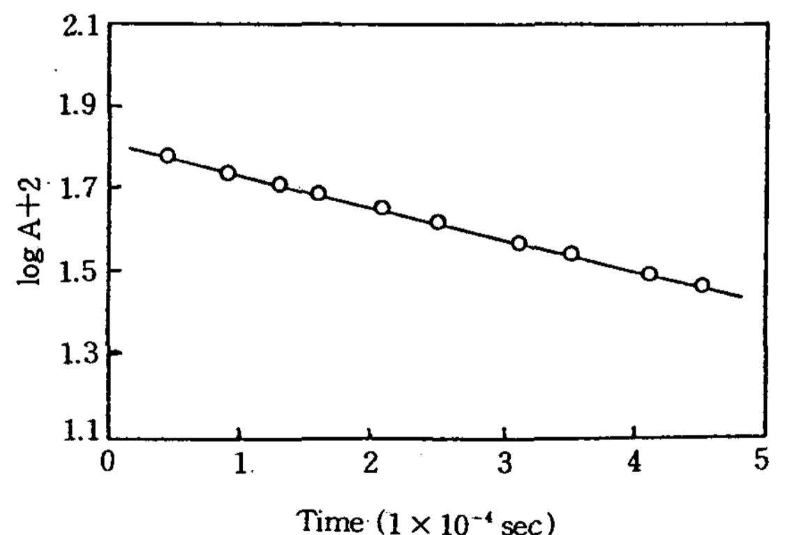
Fig. 1. The plot of log A(absorbance) vs. time for the hydrolysis of cinnamenylisophorone at pH 12.0 and 25°C
