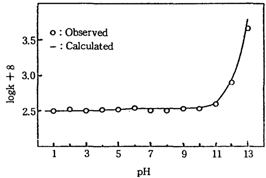
Fig. 2. pH-Rate profile for the hydrolysis of cinnamenyliosphorone at 25°C.
