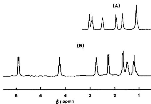
Fig. 5. ^1\text{H} NMR spectra of \text{trans-}[\text{Co}(\text{R,R-chxn})_2\text{Cl}_2]\text{BPh}_4 in \text{CD}_2\text{Cl}_2 (A) and \text{DMSO-d}_6 (B).
