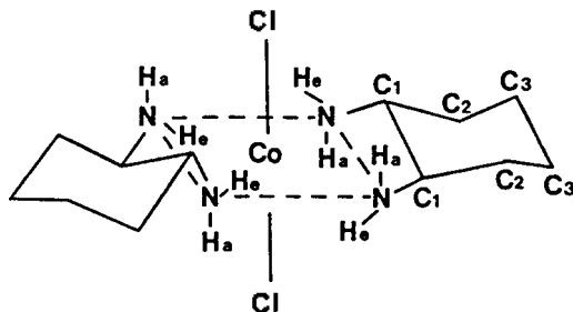
Fig. 4. Structural model of trans -[Co( R,R -chxn) 2 Cl 2 ] + complex ion. H ax and H eq denote axial and equatorial N-H protons of R,R -chxn ligand.
