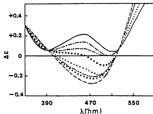
Fig. 1. The CD spectra of \text{trans-}[\text{Co}(\text{R,R-chxn})_2\text{Cl}_2]\text{Cl} ( 2 \times 10^{-3} M ) in various solvents. (----) Nitromethane, (××××) \text{H}_2\text{O} , (.....) EtOH, (.....) MeOH, (.....) Solid State, (---) DMF, (.....) DMSO, (—) Pyridine.
