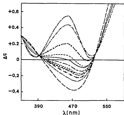
Fig. 3. The CD spectra of trans -[Co( R,R -chxn) 2 Cl 2 ] BPh 4 ( 2 \times 10^{-3} M ) in various solvents. (----) Nitromethane, (-·-·-) Nitrobenzene, (++++) Benzonitrile, (- - - -) AN, (xxxx) 1,4-Dioxane, (····) Acetone, (-·-·-) MeOH, (—) THF, (- - - -) Solid State, (-x-x) DMF, (-·-·-) DMSO, (-·-·-) Pyridine.
