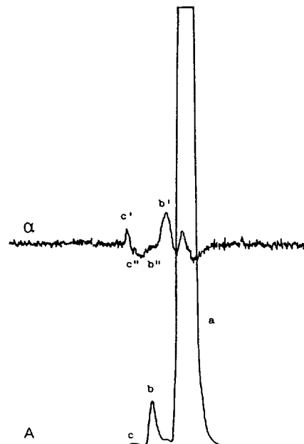
Figure 1. LC/UV/polarimeter-combination measurement of the reaction mixture of 6 with ethyl chloroformate [concentration: 1mg/ml, injection: 100 \mu l, eluent: ethanol, temp.: 22°C, pressure: ~65 bar, UV (ERC 7210): 278 nm, polarimeter (PE 241): 365 nm]*.
