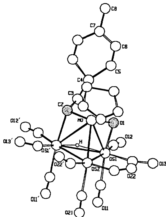
Figure 2. The molecular structure of \text{CpMoOs}_3(\text{CO})_9(\mu\text{-H})(\mu\text{-O})(\mu\text{-CHCH}_2\text{Tol}) ( 3c ) molecule. Selected bond lengths are Mo-Os(2)=2.634(6), Mo-Os(1)=2.846(3), Os(1)-Os(1')=2.983(2), Os(1)-O(1)=1.99(3), Mo-O(1)=1.87(3), Os(1)-C(2)=2.16(6), and Mo-C(2)=1.88(5) Å. The hydride ligand is shown in the predicted position.
