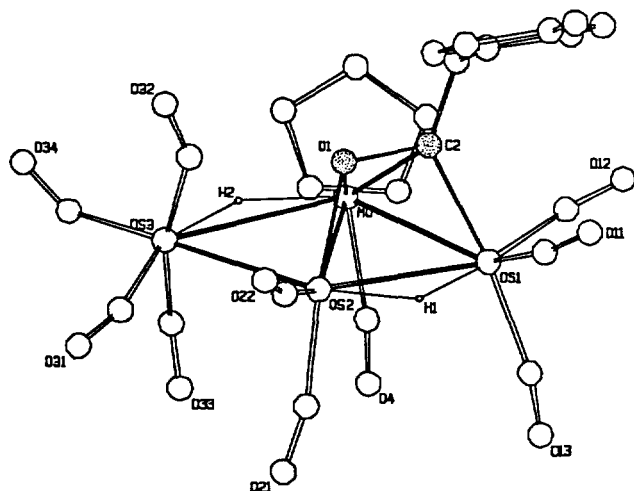
Figure 1. The molecular structure of \text{CpMoOs}_3(\text{CO})_{10}(\mu\text{-H})_2[\mu\text{-}\eta^2\text{-C}(\text{O})\text{CH}_2\text{Tol}] ( 2-A ) molecule. Intermetallic distances are Os(1)-Os(2)=2.862(3), Os(1)-Mo=2.928(7), Os(2)-Os(3)=2.799(5), Os(2)-Mo=2.763(7), and Os(3)-Mo=3.203(8) Å. Hydride ligands are shown in their predicted positions (see text).
