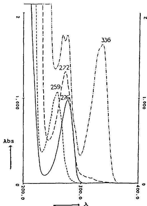
Figure 6. The absorption spectra of N-(2-haloarylmethyl)pyridinium, N-arylmethyl-2-halopyridinium salts and N-(2-haloarylmethyl) isoquinolinium salt in water. 1a ; —, 2a ; - - - - - , 3a ; - · - · - · , 5a ; - - - - - , 6 ; - · - · - · .
