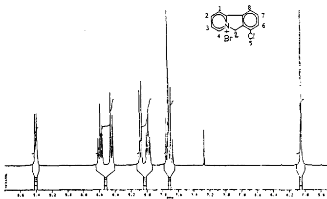
Figure 4. Proton NMR spectrum, at 300 MHz, in TFA-D+ \text{CDCl}_3 , of isoindolium salt, 3b .
