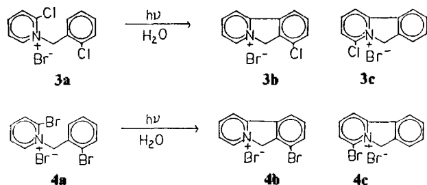
Figure 3. Intramolecular photocyclization of N-(2-halobenzyl)-2-halopyridinium salts ( 3a and 4a ).
