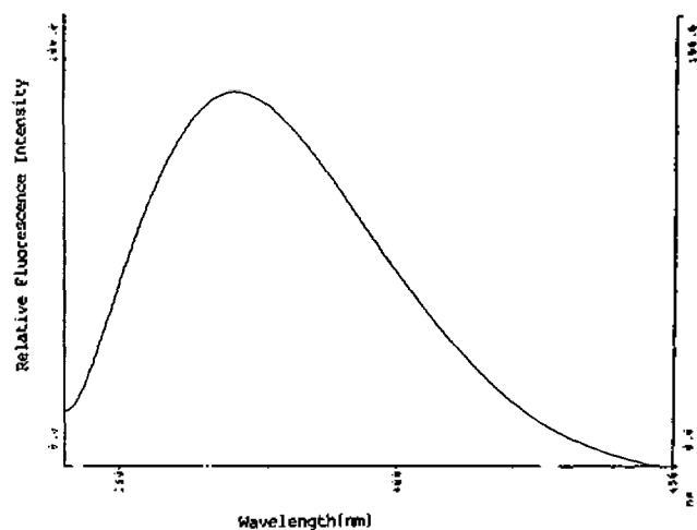
Figure 7. Fluorescence emission spectra of N-(2-chlorobenzyl)pyridinium salt (0.1 mM) in water. The excitation wavelength was 260 nm. The optical density was 0.39 at 260 nm.
