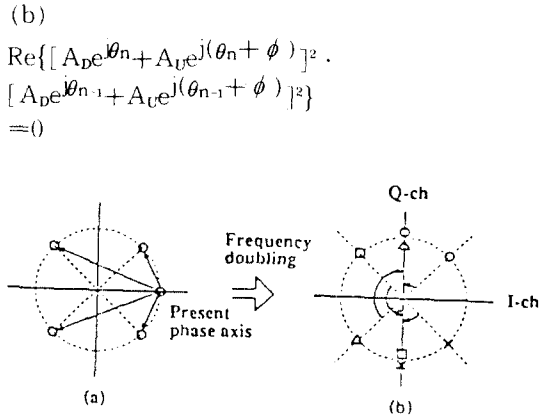
Figure 1: Frequency doubler.
