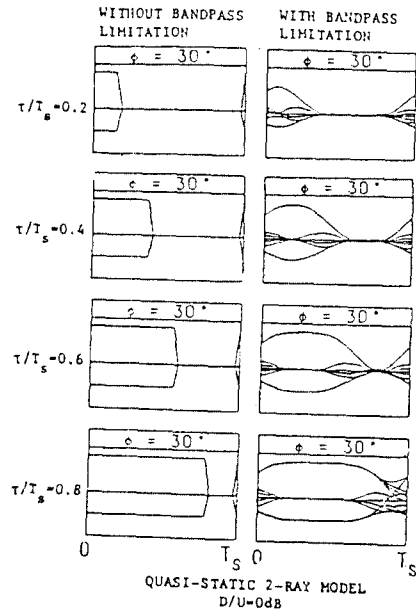
Figure 3: Eye patterns of I-ch detector output.
