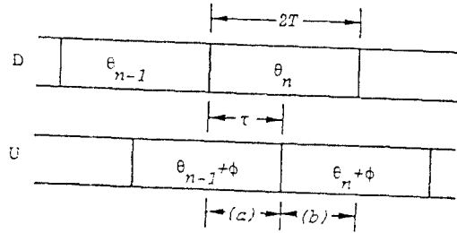
Figure 2: Carrier phase of \pi/4 shift QPSK signal in two ray multipath model.
