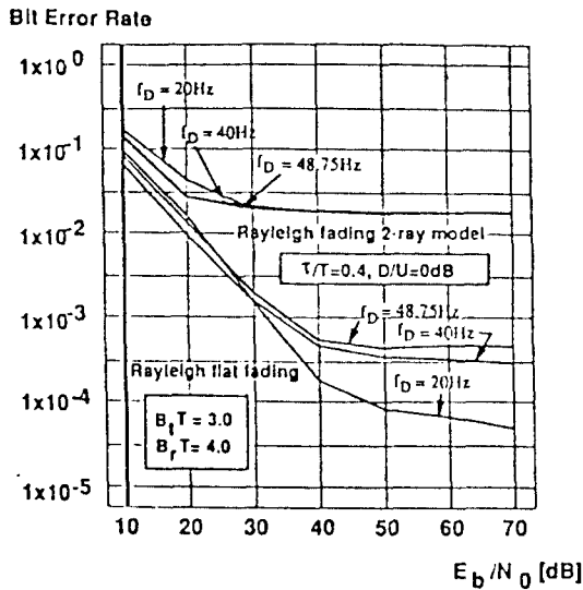
Figure 11 : BER performance under Rayleigh fading two ray model with maximum Doppler frequency as a parameter.
