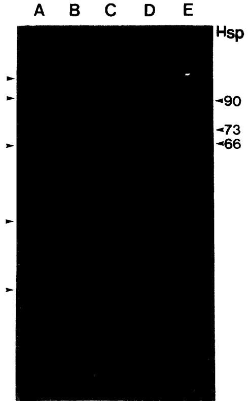
Fig. 2. Autoradiogram of the proteins synthesized in C. jejuni heat-treated at various temperatures for 15 Minutes. Lane A, 42°C; Lane B, 45°C; Lane C, 48°C; Lane D, 51°C; Lane E, 55°C. The arrowheads indicate standard molecular weight markers of 116, 97.4, 66, 45, and 25 kD, respectively, from the top.
