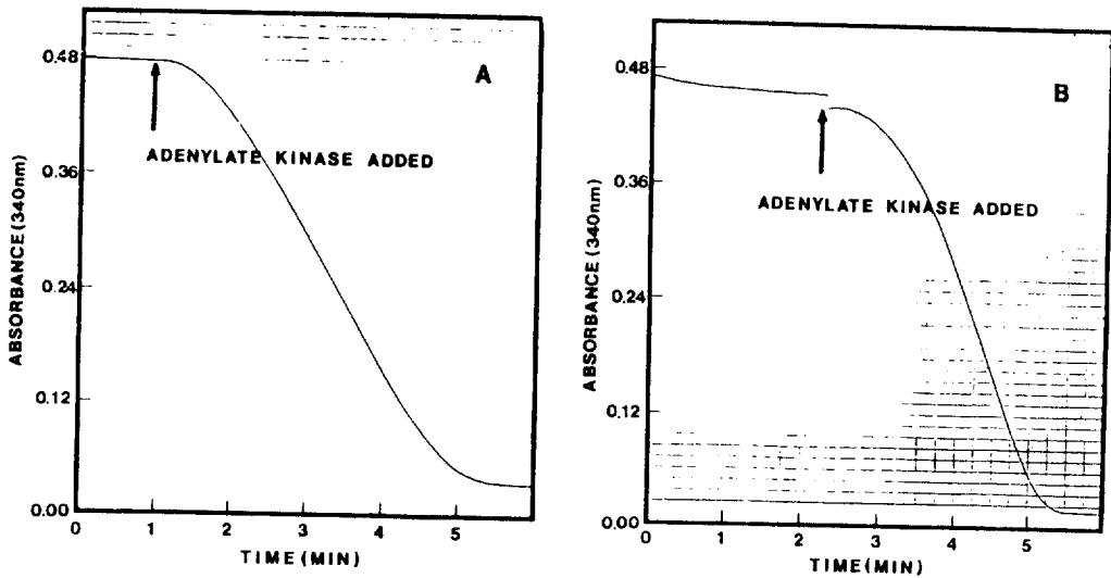
Fig. 2. Decrease in absorbance at 340 nm by the addition of adenylate kinase to malonyl-CoA synthetase/ADP coupling reaction mixture. A: R. japonicum enzyme. B: R. trifolii enzyme. The reaction mixture contained the complete malonyl-CoA synthetase reaction system containing enzyme, ATP, malonate, and CoA, and ADP coupling system containing PEP, NADH, pyruvate kinase, and lactate dehydrogenase. Decrease in absorbance at 340 nm by addition of adenylate kinase indicates the formation of ADP from AMP produced by malonyl-CoA synthetase.
