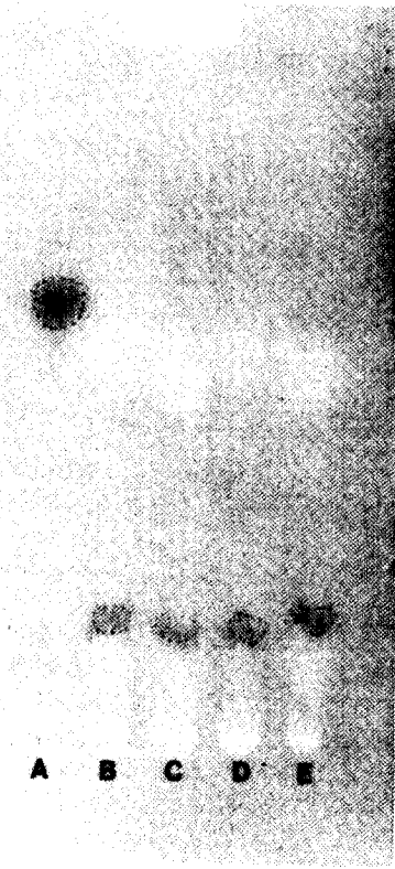
Fig. 5. Identification of the products by the amidases catalysis with paper chromatography. Developing solvent was a mixture of n -butanol, ethanol, and water (2:2:1). A: Authentic acetohydroxamate. B: Hydroxamate produced from malonamate and hydroxylamine by R. japonicum amidase. C: Hydroxamate produced from malonate and hydroxylamine by R. japonicum amidase. D: Hydroxamate produced from malonate and hydroxylamine by R. meliloti amidase, and E: Authentic malonohydroxamate.
