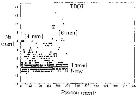
Fig. 17 Rpv stud indications (4,6 mm notch) by TDOT
