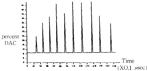
Fig. 4 Amplitude and time value of thread signal
