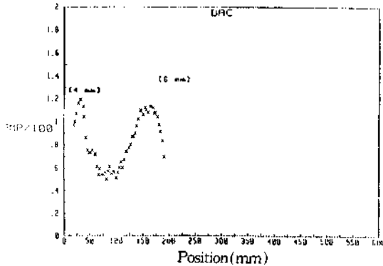
Fig. 7 Rpv stud indications (4,6mm) by DAC
