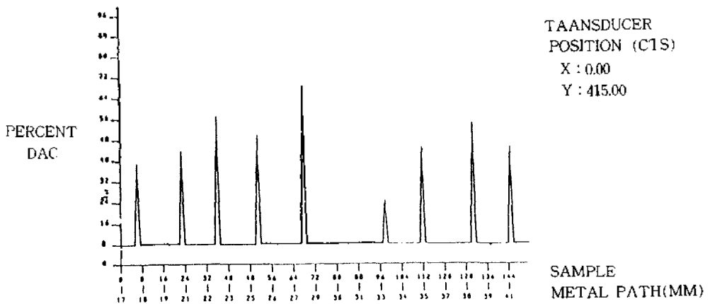
Fig. 14 Rcp stud 1.5mm notch signals by window
