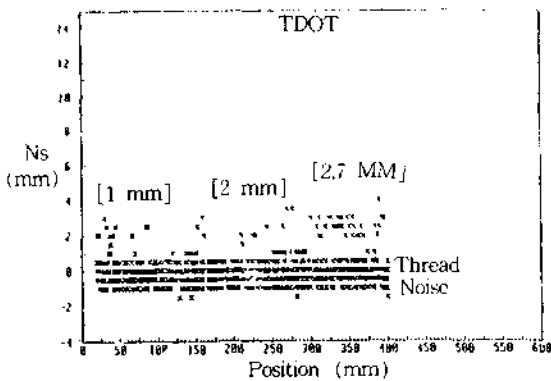
Fig. 16 Rpv stud indications (1,2,2.7 mm notch) by TDOT
