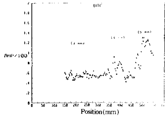
Fig. 9 Rcp stud indications (3,4,5mm) by DAC
