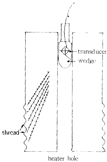
(b) angle beam
