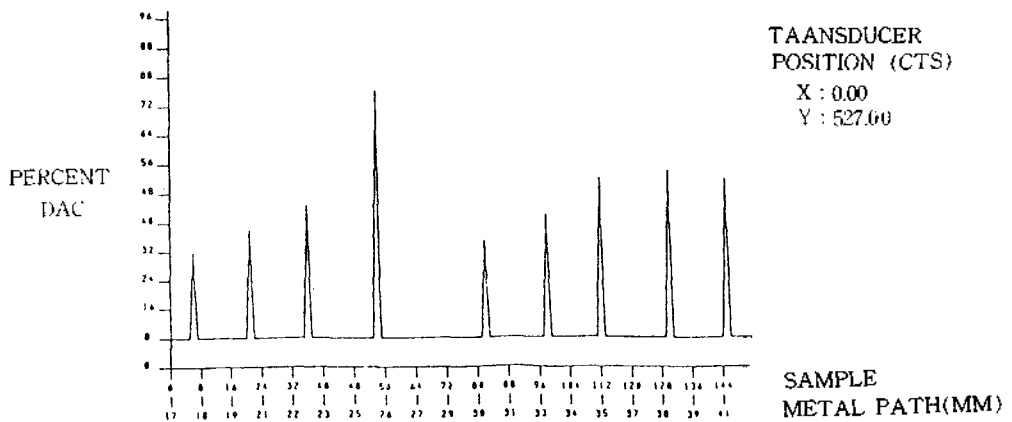
Fig. 15 Rcp stud 2mm notch signals by window
