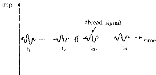
Fig. 2 Pulse train from stud(bolt) threads
