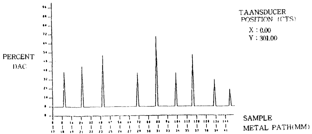
Fig. 13 Rcp stud 1mm notch signals by window
