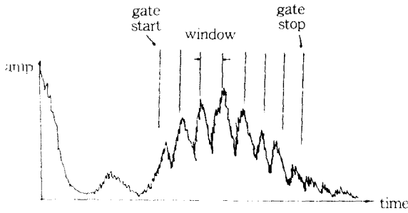
Fig. 3 Gating and windowing of thread signal
