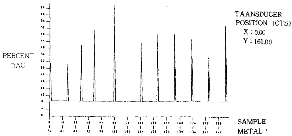
Fig. 11 Rpv stud 2mm notch signals by window
