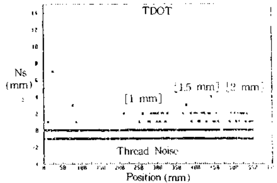
Fig. 18 Rep stud indications (1,1.5,2 mm notch) by TDOT
