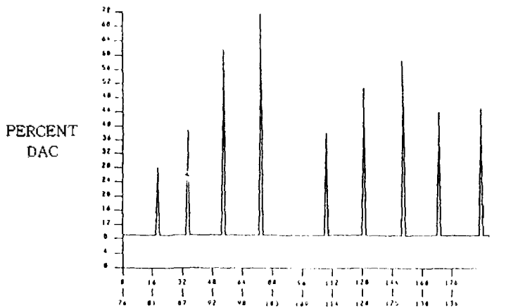
Fig. 12 Rpv stud 2.7mm notch signals by
