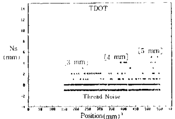
Fig. 19 Rcp stud indications (3,4,5 mm notch) by TDOT
