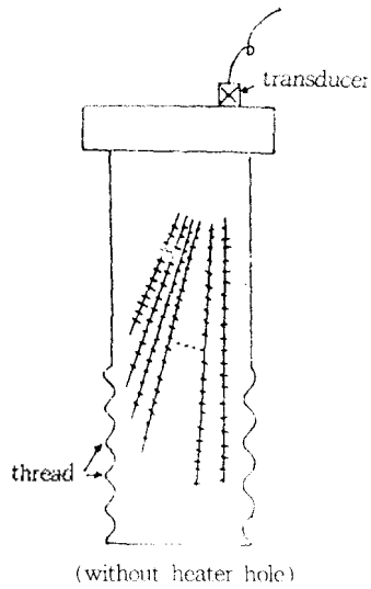
(a) straight beam
