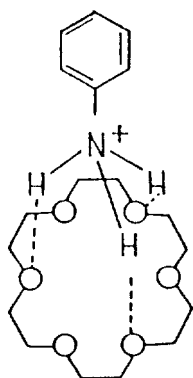
Figure 6. Diagrammatic representations of binding of anilinium ion to 18-crown-6. 8 Dashed lines indicate hydrogen bonds.
