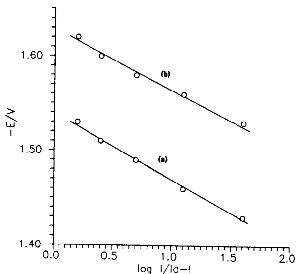
Figure 2. Plots of -E vs. \log [I_d - I] for (a) 3,5-dimethylanilinium ion and (b) its complex with 18-crown-6 in methanol at 25.0^\circ\text{C} .
