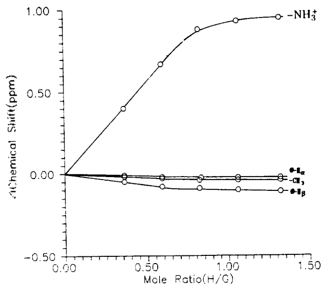
Figure 10. Proton chemical shift of 0.05 M 4-methylanilinium ion at various host/guest mole ratio in \text{CDCl}_3/\text{DMSO} (10:1 v/v).
