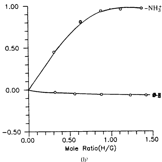
Figure 9. Proton chemical shift of (a) 0.05 M 18-crown-6 at various guest/host mole ratio and (b) 0.05 M anilinium ion at various host/guest mole ratio in \text{CDCl}_3/\text{DMSO} (10:1 v/v).
