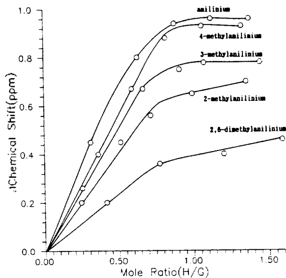
Figure 11. Proton chemical shift of ammonium of guest ion at various host/guest mole ratio in \text{CDCl}_3/\text{DMSO} (10:1 v/v).
