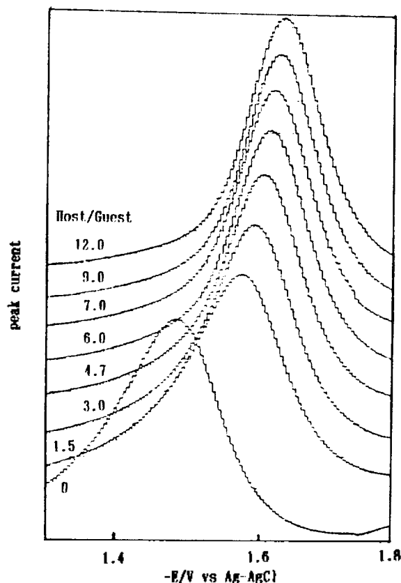
Figure 3. Differential pulse polarograms of 1.0 \times 10^{-3} M anilinium ion at various host/guest mole ratio in methanol at 25.0^\circ\text{C} .
