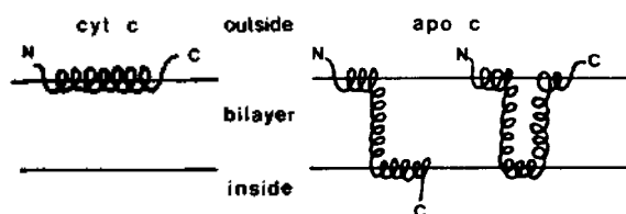
Figure 3. Mode of topologies of Cyt c and Apo c in the vesicle bilayer.
