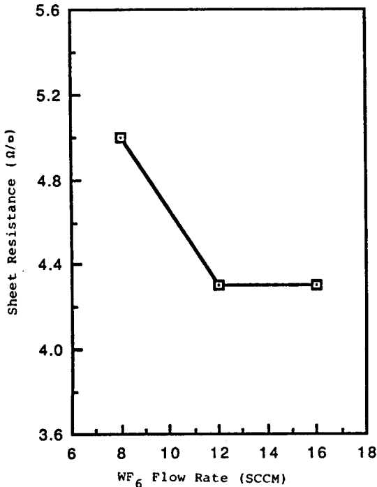
Fig. 8. Sheet resistance of WSi 2 film after oxidation.
