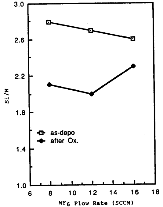
Fig. 6. Composition changes in WSi_x film depending on the flow rate of WF_6 .
