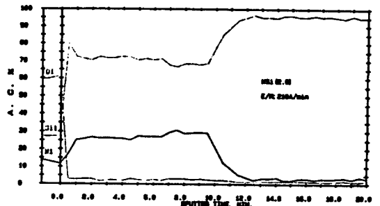
Fig. 3. Auger depth profile for the WSi 3 film annealed at 900°C for 40min.
