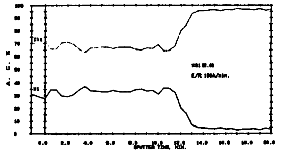
Fig. 4. Auger depth profile for the WSi 3 film oxidized at 900°C for 20min.
