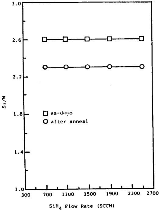
Fig. 5. Composition changes in WSi_x film depending on the flow rate of SiH_4 .
