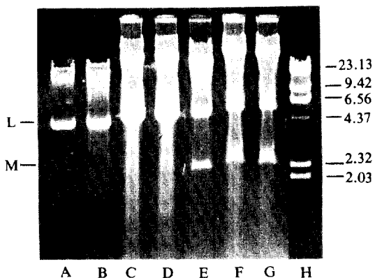
Fig. 8. Agarose gel electrophoresis of dsRNA from yeast strains. A; K 52-T 6, B; K 52-C 4, C; FC-105, D; FC-260, E; K 52, F; FWKS 105, G; FWKS 260, H; Lambda DNA (Hind III), Number; DNA length (kb), L; High molecular weight species, M; Low molecular weight species.
