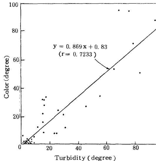
Fig. 2. The Regression Line of Turbidity and Color
