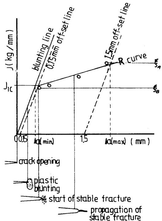
Fig. 11 Schematic drawing of static fracture blunting line, R curve and J 1c
