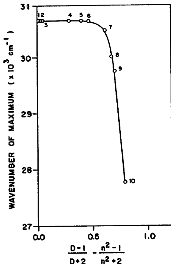
Figure 2. Solvent shifts of 1st absorption band of piroxicam for the solvents: (1) hexane; (2) \text{CCl}_4 ; (3) dioxane; (4) chloroform; (5) ethylacetate; (6) dichloromethane; (7) butanol; (8) ethanol; (9) methanol and (10) \text{H}_2\text{O} .
