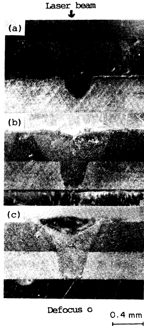
Fig. 6. Longitudinal sections of SK-5/SUS 304 plates (0.4/0.4mm) spot-welded under various laser powers. (a) 24J/pulse, (b) 30J/pulse, (c) 37.5J/pulse
