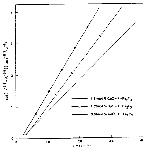
Figure 2. Comparative rates of CO oxidation on various \text{CoO}-\alpha\text{-Fe}_2\text{O}_3 at 420^\circ\text{C} . P_{\text{CO}} = 50 torr; P_{\text{O}_2} = 25 torr; each catalyst = 1 g (100-160 mesh); P_0 , total initial pressure; P , total pressure.
