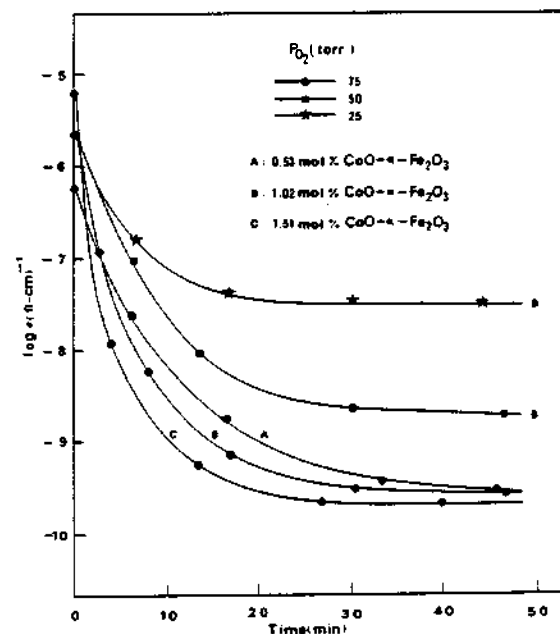
Figure 6. P_{O_2} dependences of conductivity for various mol % CoO- \alpha -Fe 2 O 3 as a function of time at 350°C.
