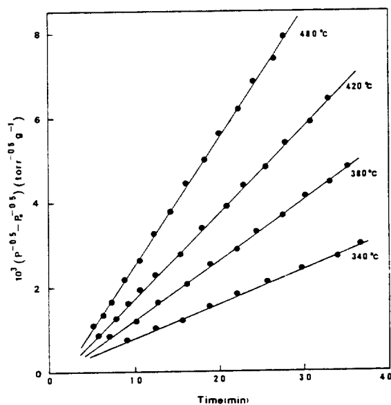
Figure 1. Oxidation rates of carbon monoxide on 0.53 mol % \text{CoO}-\alpha\text{-Fe}_2\text{O}_3 at various temperatures. P_{\text{CO}} = 50 torr; P_{\text{O}_2} = 25 torr; catalyst = 1g (100-160 mesh); P_0 , total initial pressure; P , total pressure.
