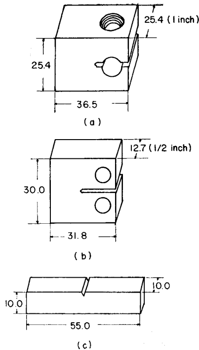
Fig. 2. Fracture Toughness Test Specimens. (a) 1 T WOL Specimen, (b) ASTM E-399 Type 1/2T C/T Specimen, (c) ASTM E-23 Type Charpy Impact Test Specimen.
