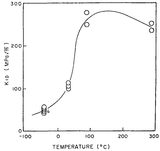
Fig. 11. Variations of the Dynamic Fracture Toughness:K 1d from the Instrumented Precracked Charpy Impact Test with Temperature.
