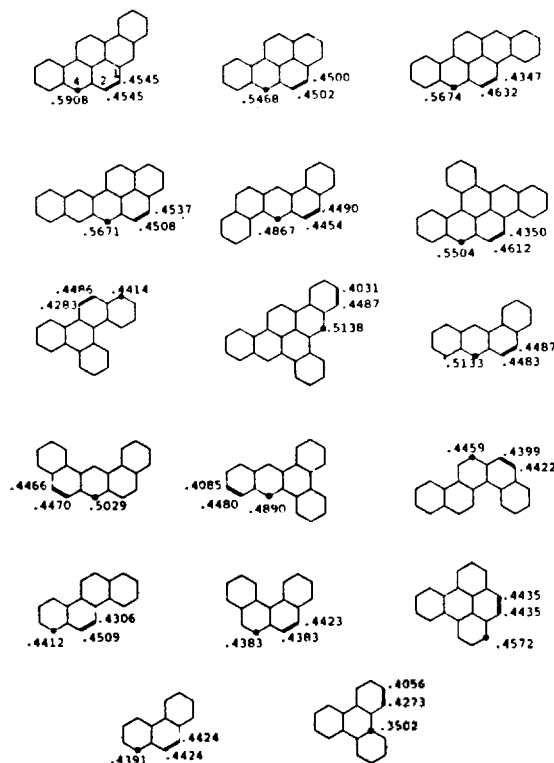
Chart 2. Self-atom polarizability( \pi_{ii} ) of the trans 1,2,4 region for PAH's.
