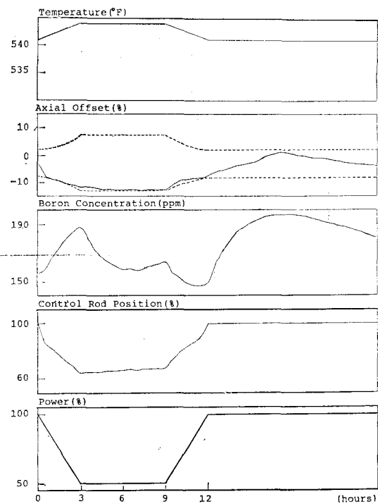
Fig. 3. 12-3-6-3 Load-Follow with SPINR Mode (KNU-1, CY1, 85% EOL)
