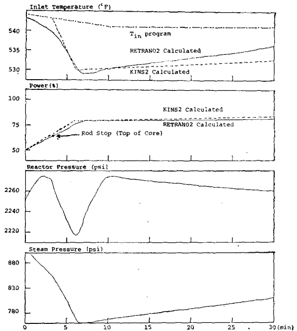
Fig. 4. Return-to Power with Reduced Temperature
