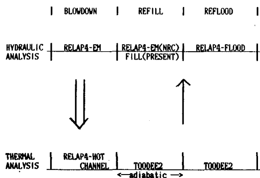
Fig. 1. LOCA Analysis Scheme
