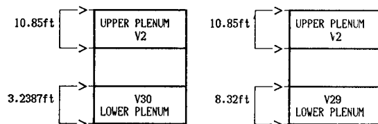
Fig. 3. Gravitational Heads through Various Volumes
