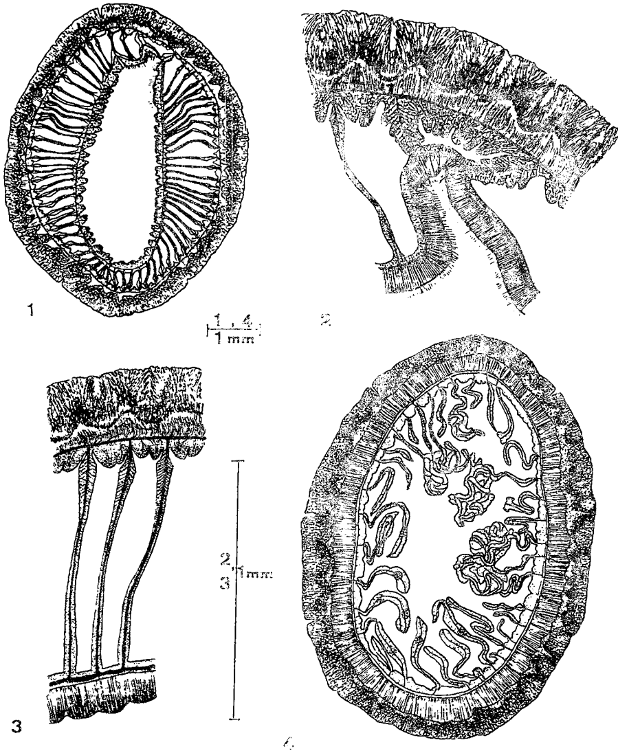
Fig. 1. Cross section through the actinopharynx. Fig. 2. A siphonoglyph with directives (dm) and a protomesentery (p2), through the actinopharynx. Fig. 3. Three metemesenteries (M, m, B), through the actinopharynx. Fig. 4. Cross section below the actinopharynx.
