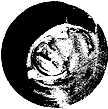
Fig. 14. Fracture surface of a dissimilar steel friction weld between SKH9 and SPS3 due to torsion test after quenching and tempering.
