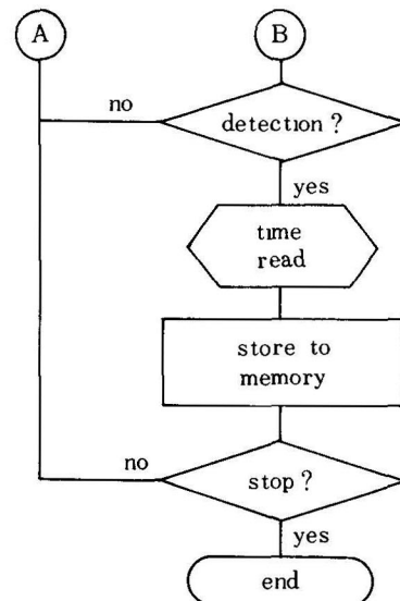
Fig. 2. General algorithm
