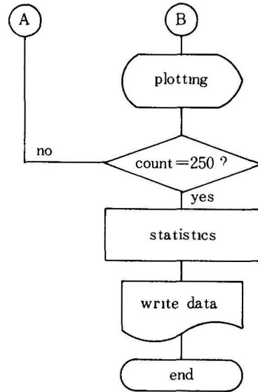
Fig. 2. General algorithm
