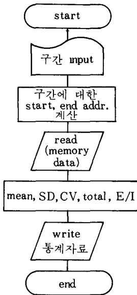
Fig. 4. Calculating algorithm
