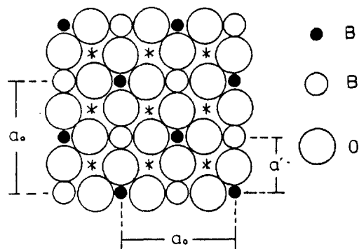
Figure 1. Rock salt arrangement of B and B' cations in the (100) plane of the cubic perovskite structure for A(B 1-x B' x )O 3 . Lattice constant a' and dimension of superlattice a 0 are shown. Asterisks stand for the A-sites.
