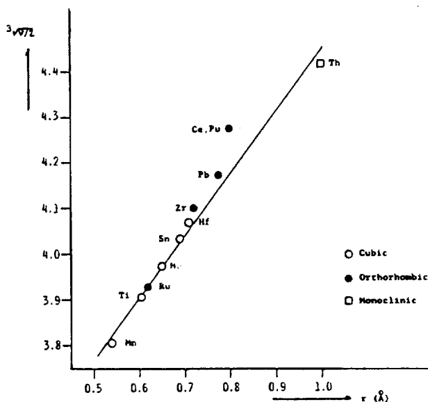
Figure 4. The linear relation between cube root of cell volume for formula unit ( \sqrt[3]{V/Z} ) vs ionic radius of M^{2+} ion for perovskites SrM^{2+}O_3 .
