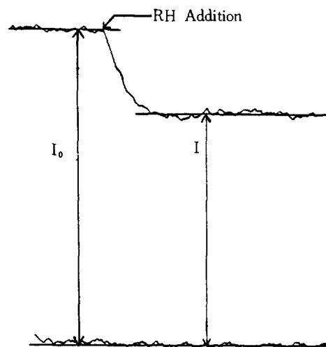
Figure 5. Mass Spectrometric Measurement of Br Atom Concentration for Kinetics. I_0 , Br Atom Intensity without the addition of RH, I , Br Atom Intensity with the addition of RH.
