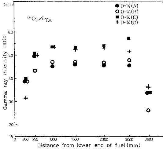
Fig. 4. Relative Burnup Distributions of Assembly D-14 (Side)
