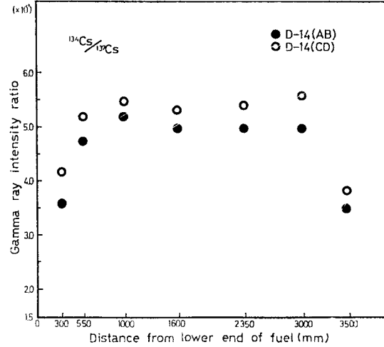
Fig. 5. Relative Burnup Distributions of Assembly D-14 (Diagonal)
