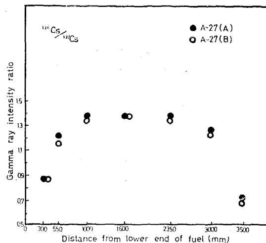
Fig. 3. Relative Burnup Distributions of Assembly A-27
