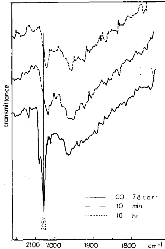
Fig. 9. IR spectra for 14% Ni sample after pumping.
