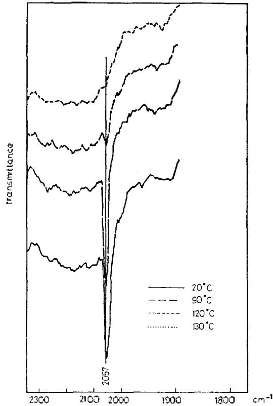
Fig. 13. IR spectra of Ni(CO) 4 adsorbed on silica gel.
