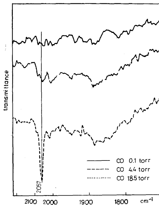
Fig. 2. IR spectra of increasing CO on 3% Ni sample at 20°C.
