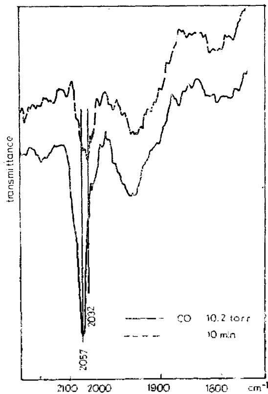
Fig. 7. IR spectra for 9.5% Ni sample after pumping.
