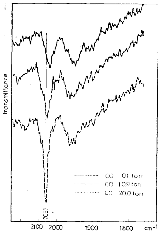
Fig. 10. IR spectra of increasing CO on 20% Ni sample at 20°C.
